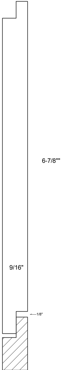
Shiplap 1x8 6-7/8" Face with 1/8" Gap
