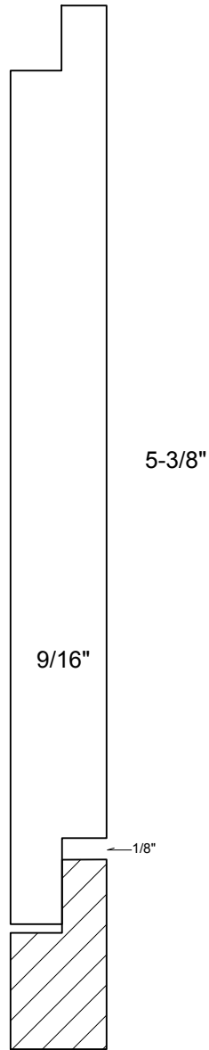
Shiplap 1x6 4-7/8" Face with 1/8" Gap
